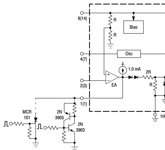
Figure 31. Latched Shutdown
