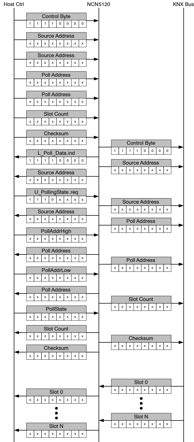
Figure 58. Master Polling Frame Service
