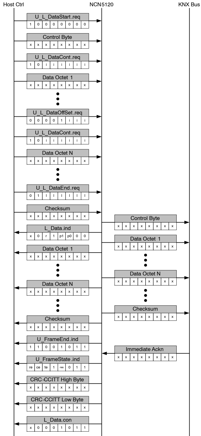
Figure 50. Send Frame, All Modes, Frame End with MARKER and with CRC-CCITT
