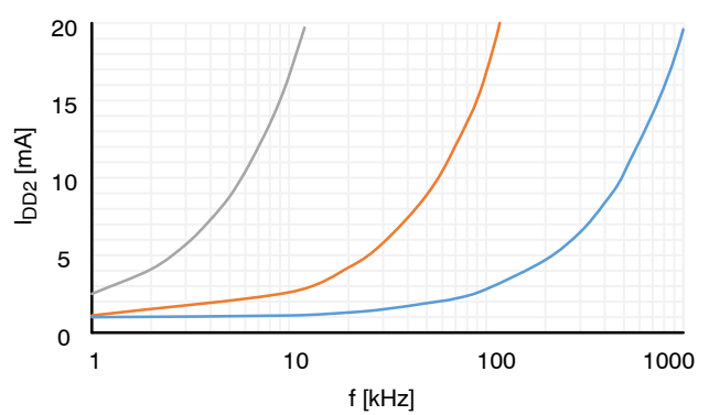
Figure 13. I_{DD2} Supply Current V_{DD2} = 15\text{ V}
