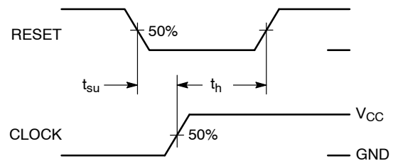
Figure 7. HC163A Only
