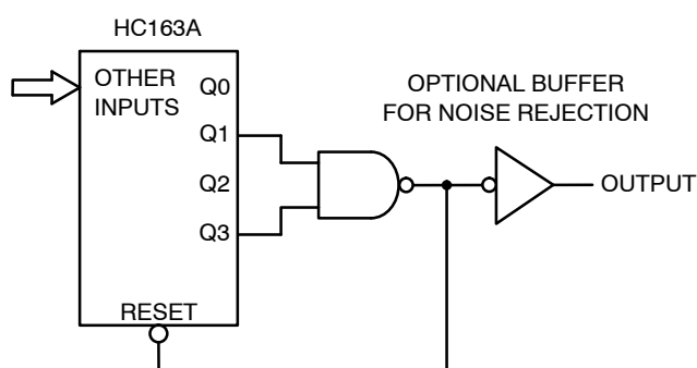
Figure 17. Modulo-11 Counter
