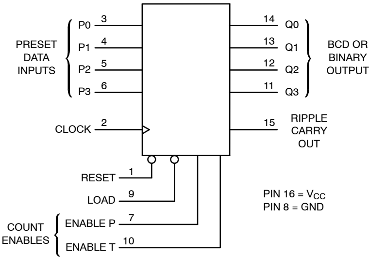
Figure 2. Logic Diagram
