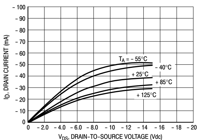
Figure 7. V_{GS} = -15 Vdc
