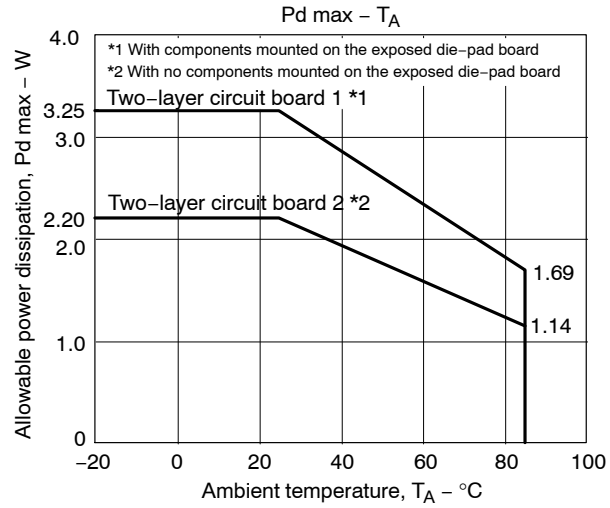
Figure 1. Power Dissipation vs Ambient Temperature Characteristic
