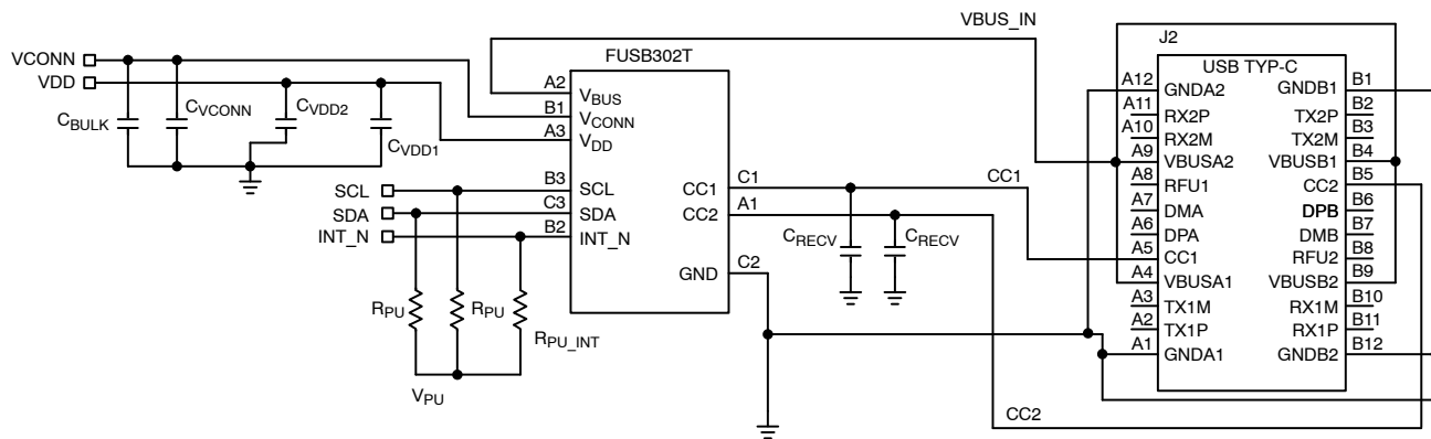
Figure 16. FUSB302T Reference Schematic Diagram
