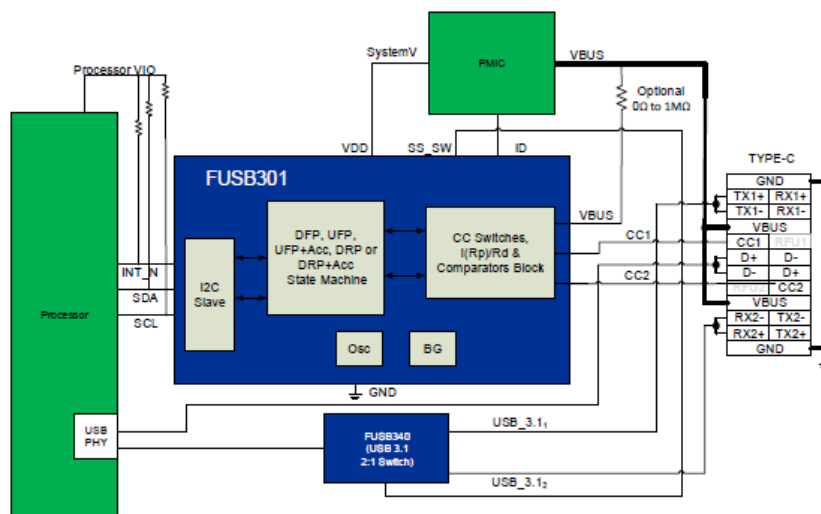
Figure 1. Typical Application
