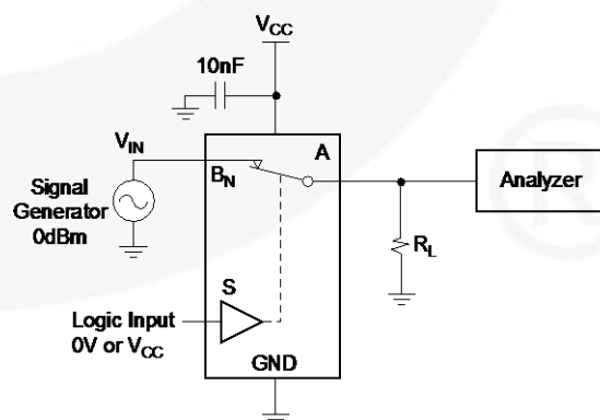
Figure 10. Harmonic Distortion
