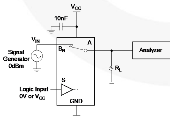
Figure 9. Bandwidth
