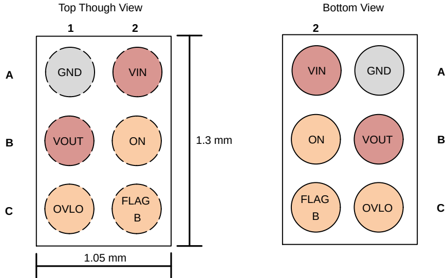
Figure 2. Pin Assignments
