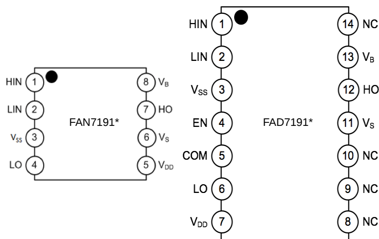
Figure 5. Pin Assignments (Top View)
