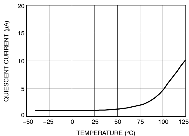
Figure 10. Quiescent Current vs. Temperature
