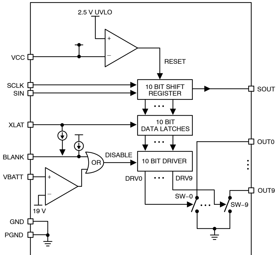
Figure 2. Block Diagram
