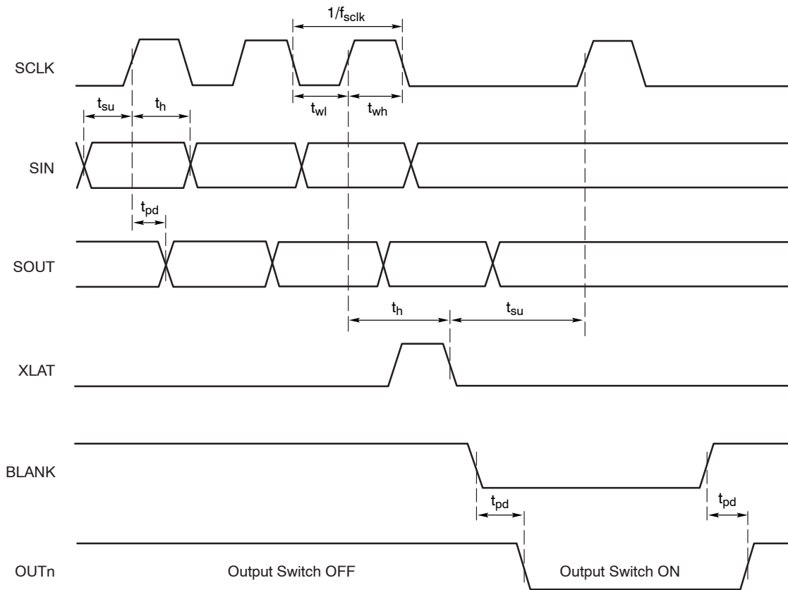
Figure 13. Timing Diagram
