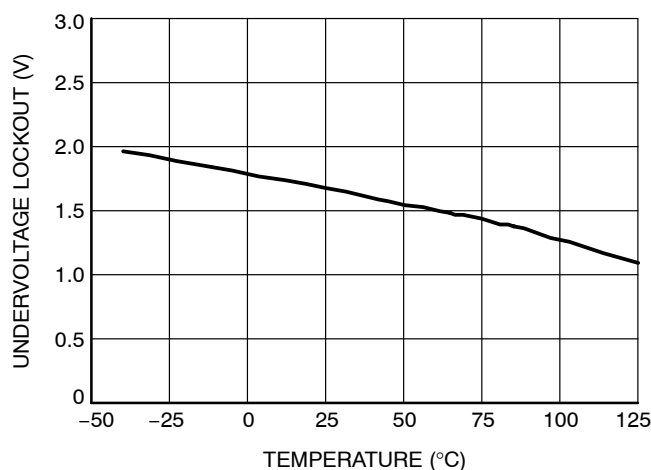
Figure 12. VCC Undervoltage Lockout vs. Temperature
