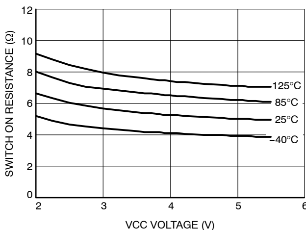
Figure 8. Switch On-resistance vs. VCC
