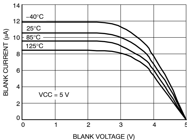
Figure 6. BLANK Pull-up Current vs. Input Voltage
