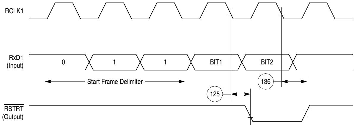
Figure 63. CAM Interface Receive Start Timing Diagram
