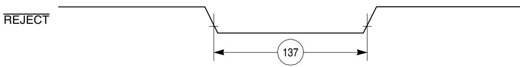
Figure 64. CAM Interface \overline{\text{REJECT}} Timing Diagram
