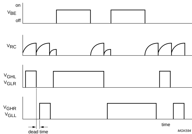
Fig.3 Timing diagram.
