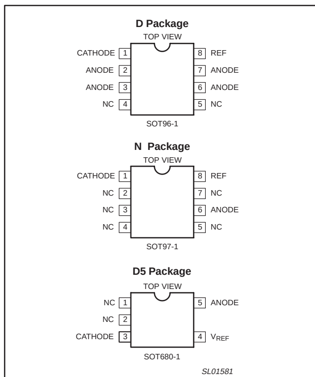
Figure 1. Pin configuration.
