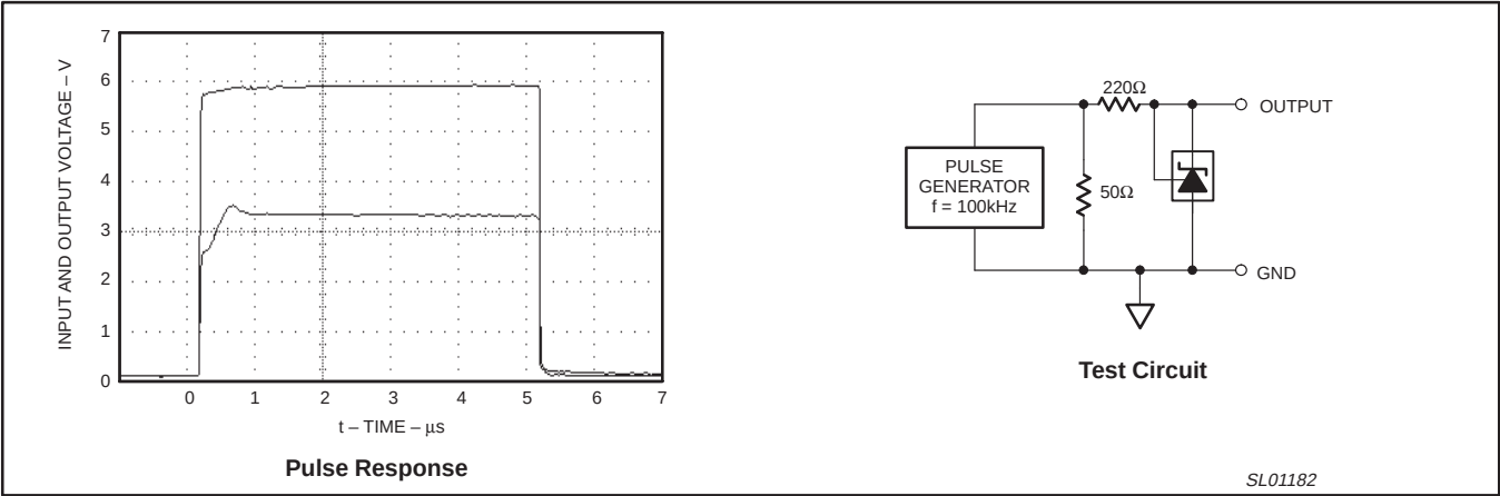
Figure 14. Pulse Response
