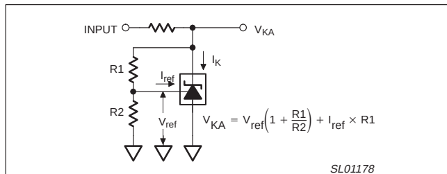
Figure 4. Test Circuit for V_{KA} > V_{ref}
