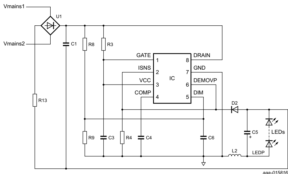
Fig 3. SSL5235BTE basic application diagram
