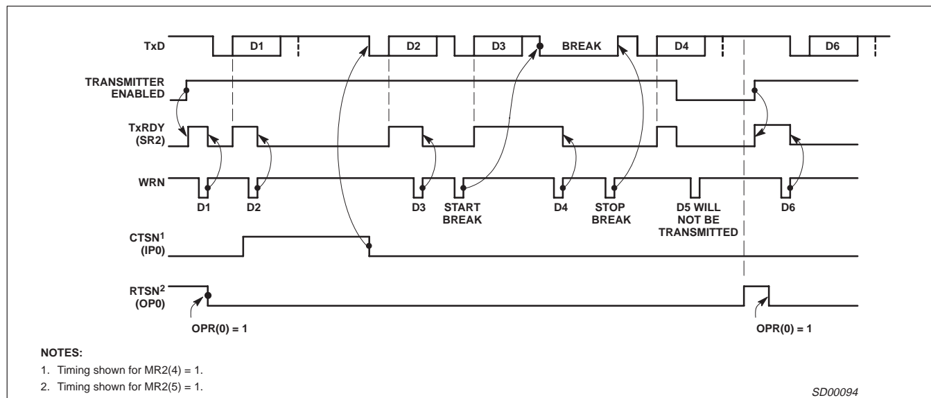
Figure 10. Transmitter Timing
