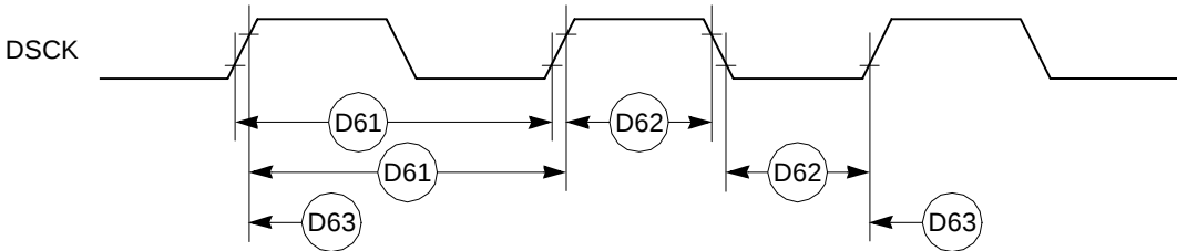
Figure 31. Debug Port Clock Input Timing
