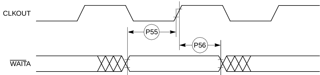
Figure 28. PCMCIA \overline{\text{WAIT}} Signals Detection Timing
