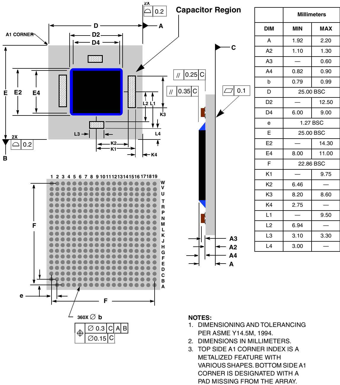
Figure 19. Mechanical Dimensions and Bottom Surface Nomenclature for the MPC7410, 360 HCTE_LGA Package
