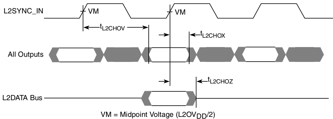
Figure 9. L2 Bus Output Timing Diagrams
