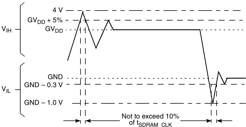
Figure 2. Overshoot/Undershoot Voltage
