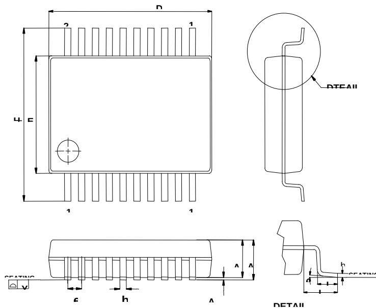
SHRINK SMALL OUTLINE PACKAGE DIMENSIONS
