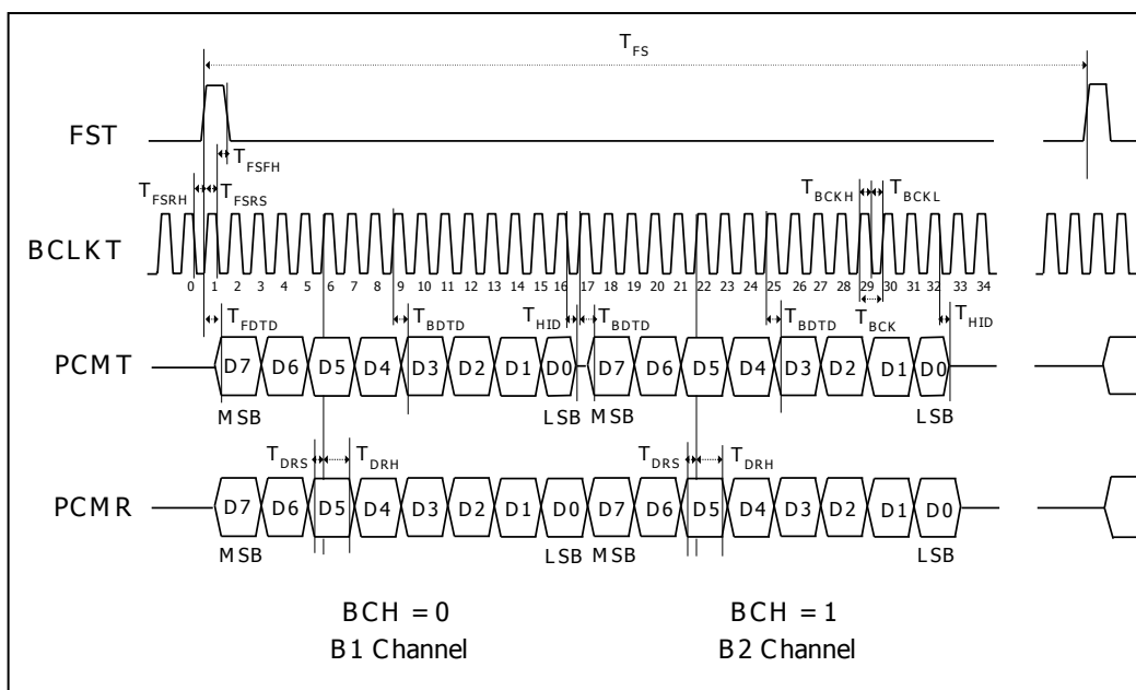
Figure 8.4 GCI PCM Timing
