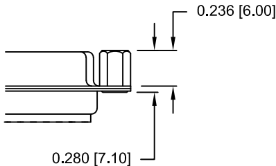
03X..... 0.236" (MATING SIDE)
