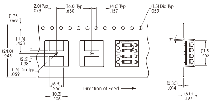
Tape Dimensions for JS0204AP4-R
