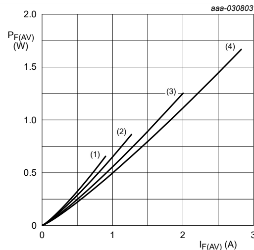
T_j = 175^\circ\text{C} (1) \delta = 0.1 (2) \delta = 0.2 (3) \delta = 0.5 (4) \delta = 1 ; DC
