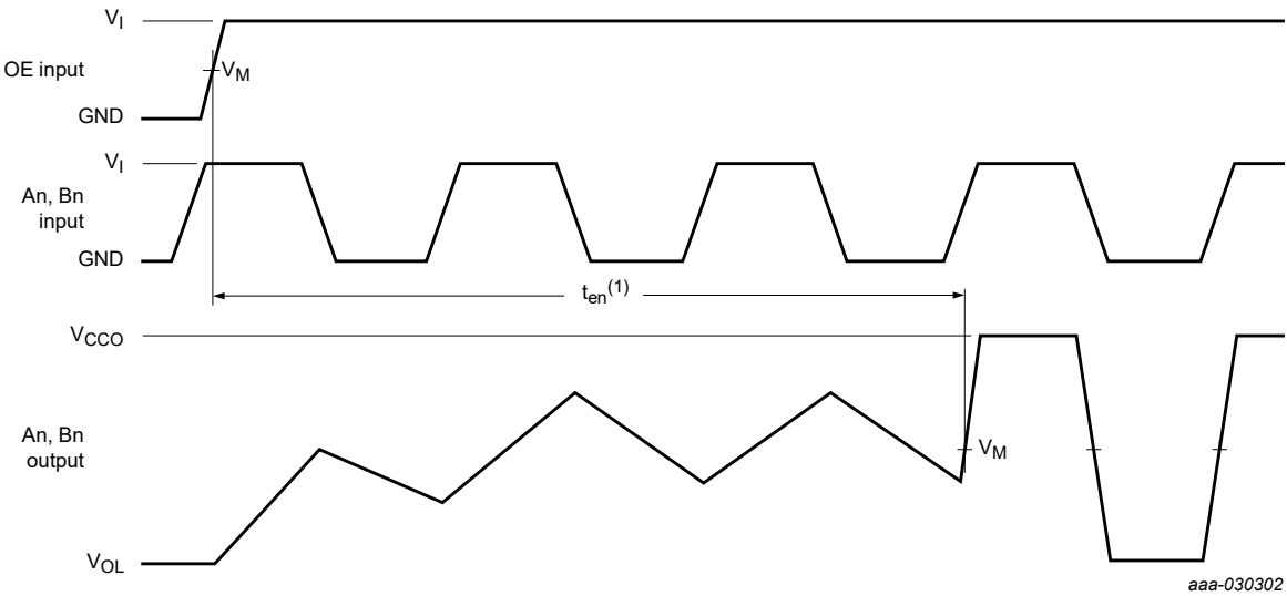
(1) The enable time ( t_{en} ) indicates the amount of time the user must allow for one one-shot circuitry to become operational after OE is taken HIGH. See also Section 12.6 Measurement points are given in Table 14 . V_{OL} is a typical output voltage level that occur with the output load. V_{CCO} is the supply voltage associated with the output.
