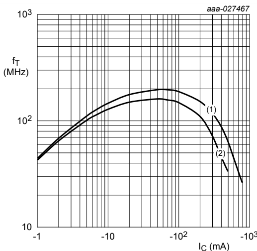
f = 100\text{ MHz}; T_{amb} = 25\text{ }^{\circ}\text{C} (1) V_{ce} = -5\text{ V} (2) V_{ce} = -1\text{ V} Figure 42. BC807K-40: Transition frequency as a function of collector current voltage; typical values
