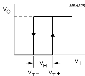
Fig.6 Transfer characteristic.
