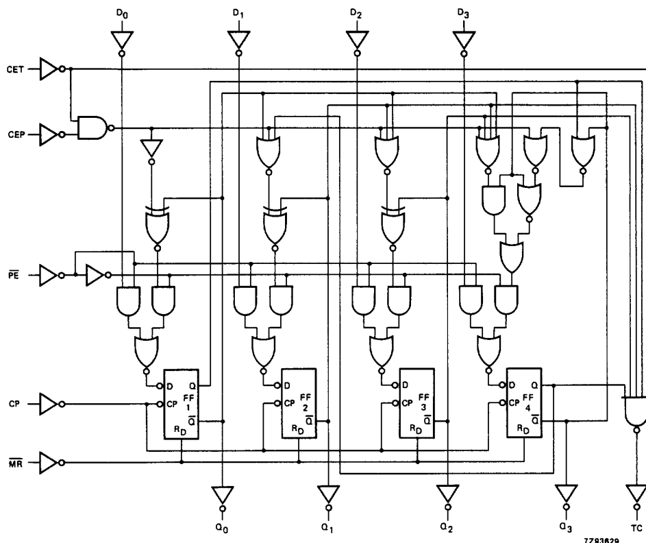
Fig.7 Logic diagram.
