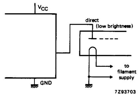
Fig.15 Connection to fluorescent display readout.
