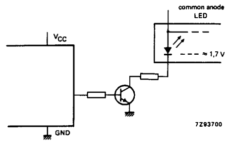
Fig.13 Connection to common anode LED display readout.
