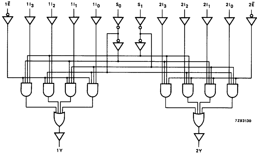
Fig.5 Logic diagram.
