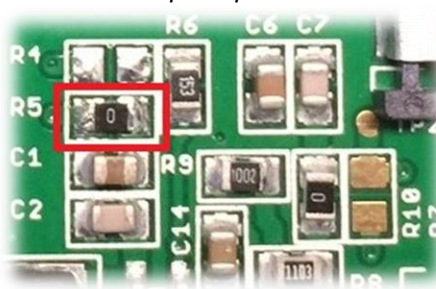
Jumper Option #1
