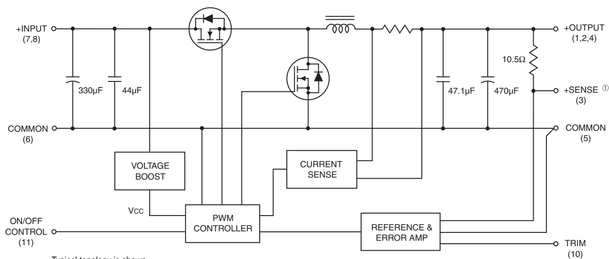
Figure 1. Simplified Schematic
