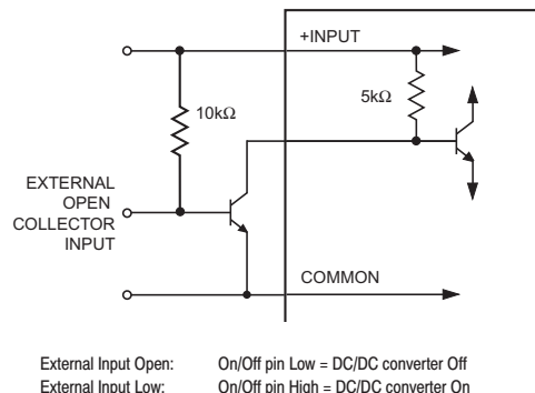
Figure 5. Driving the External Power-Up Open Collector
