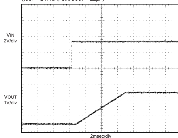
Start-Up from Vin (I OUT = 2V/10A, C IN /C OUT = 22μF)
