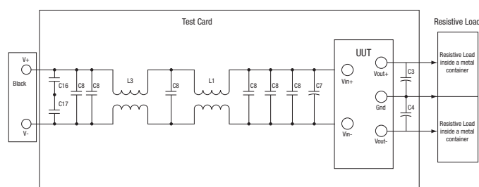
Figure 4. Conducted Emissions Test Circuit
