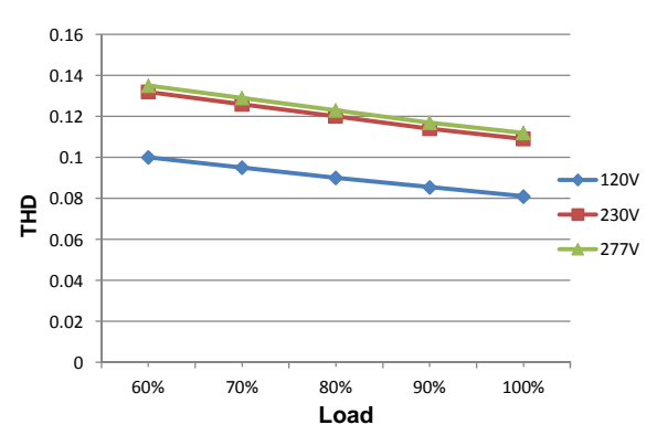
THD Curve
