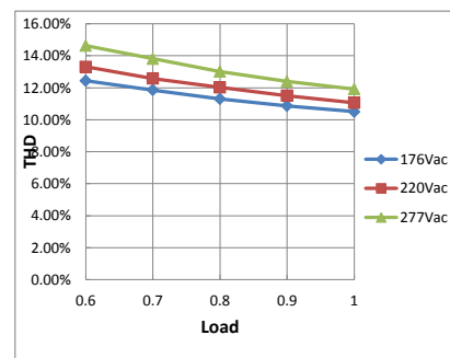
THD Curve
