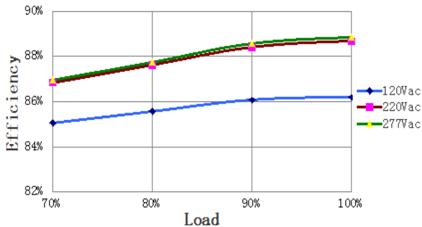
Efficiency Curve
