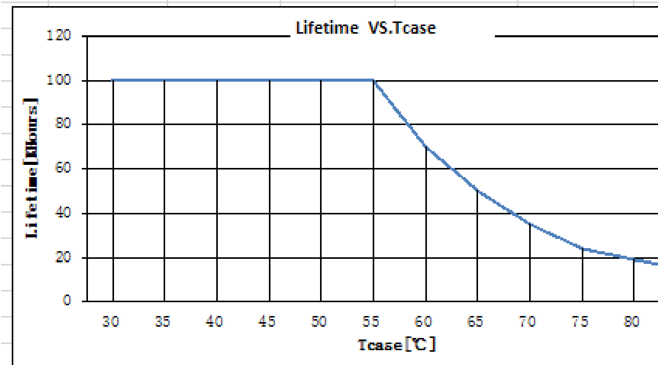
Lifetime VS.Tcase
