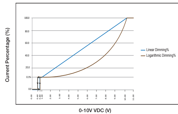
0-10V Curve
