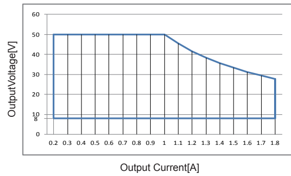
V/I OPERATING RANGE
