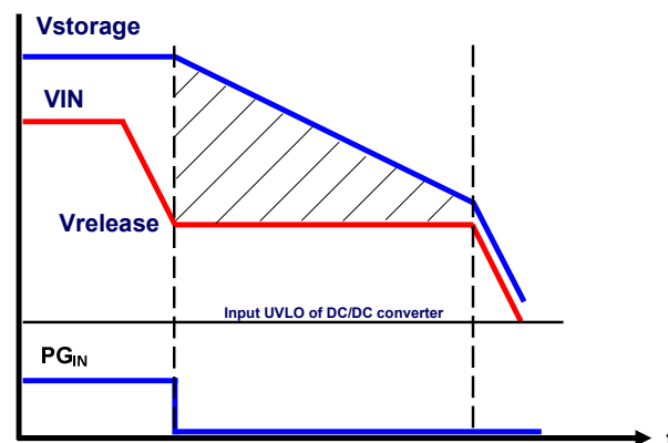
Figure 2—Timing of Releasing
