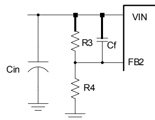
Figure 5—Feedback Circuit for Release Voltage
