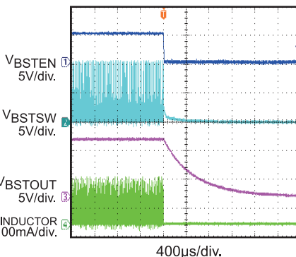
V_{BSTEN} Power Off
