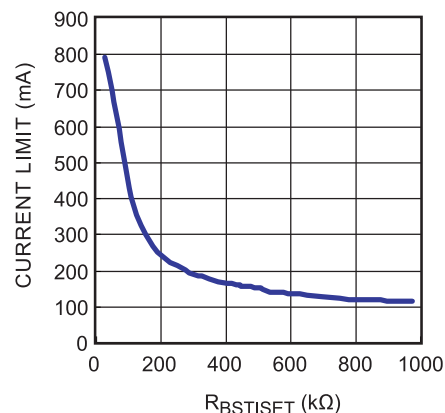
R_{BSTSET} vs. Current Limit
