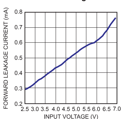
Forward Leakage Current
