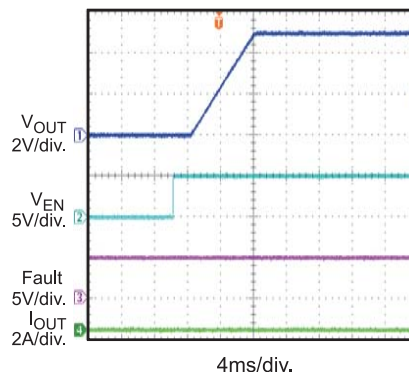
Start-Up through EN No Load
