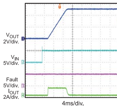
Start-Up through Input Voltage No Load, C_{OUT} = 2200\mu F
