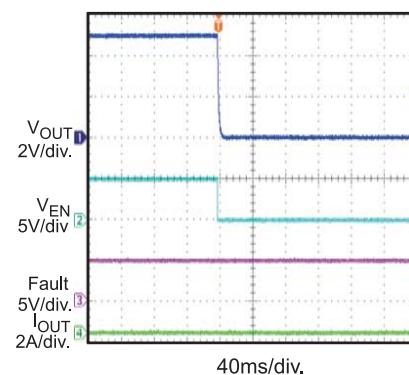
Shutdown through EN No Load
