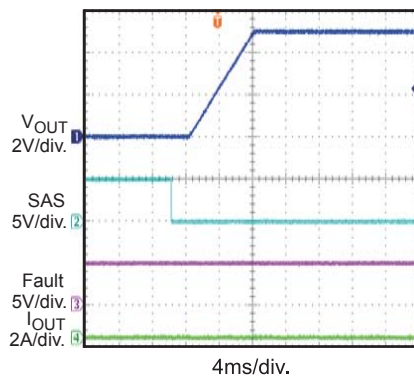
Start-Up through SAS
