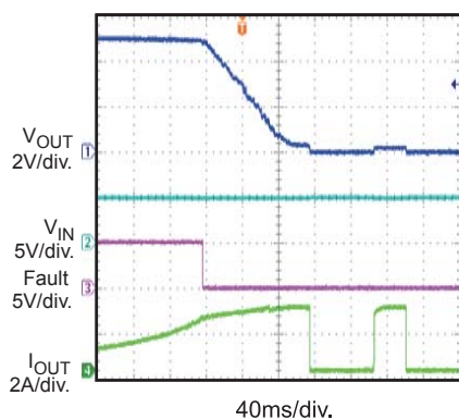
Over-Current Protection
