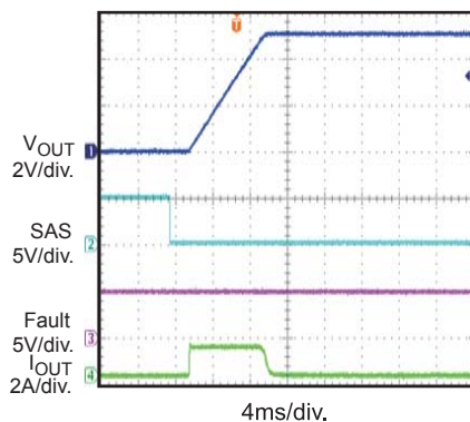
Start-Up through SAS
