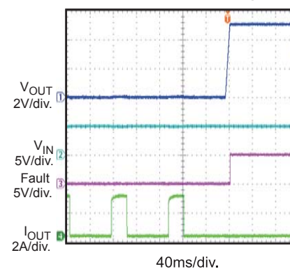
Short-Circuit Protection Recovery
