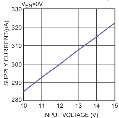
Supply Current, Output Disable vs. Input Voltage
