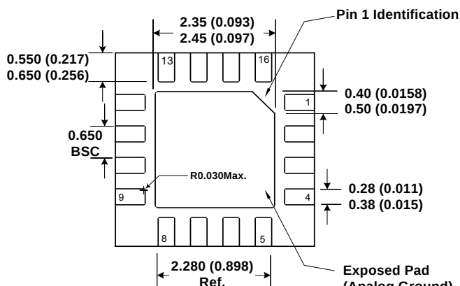
Btm View
