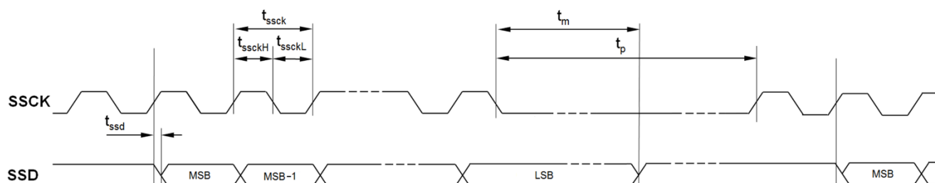
Figure 15: SSI Timing
