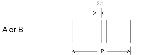
Figure 25: ABZ Jitter
