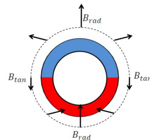
Figure 16: Side-Shift Field
