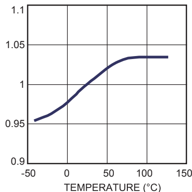
Oscillator Frequency vs. T_J
