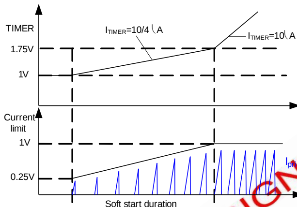
Figure 6: Soft-Start
