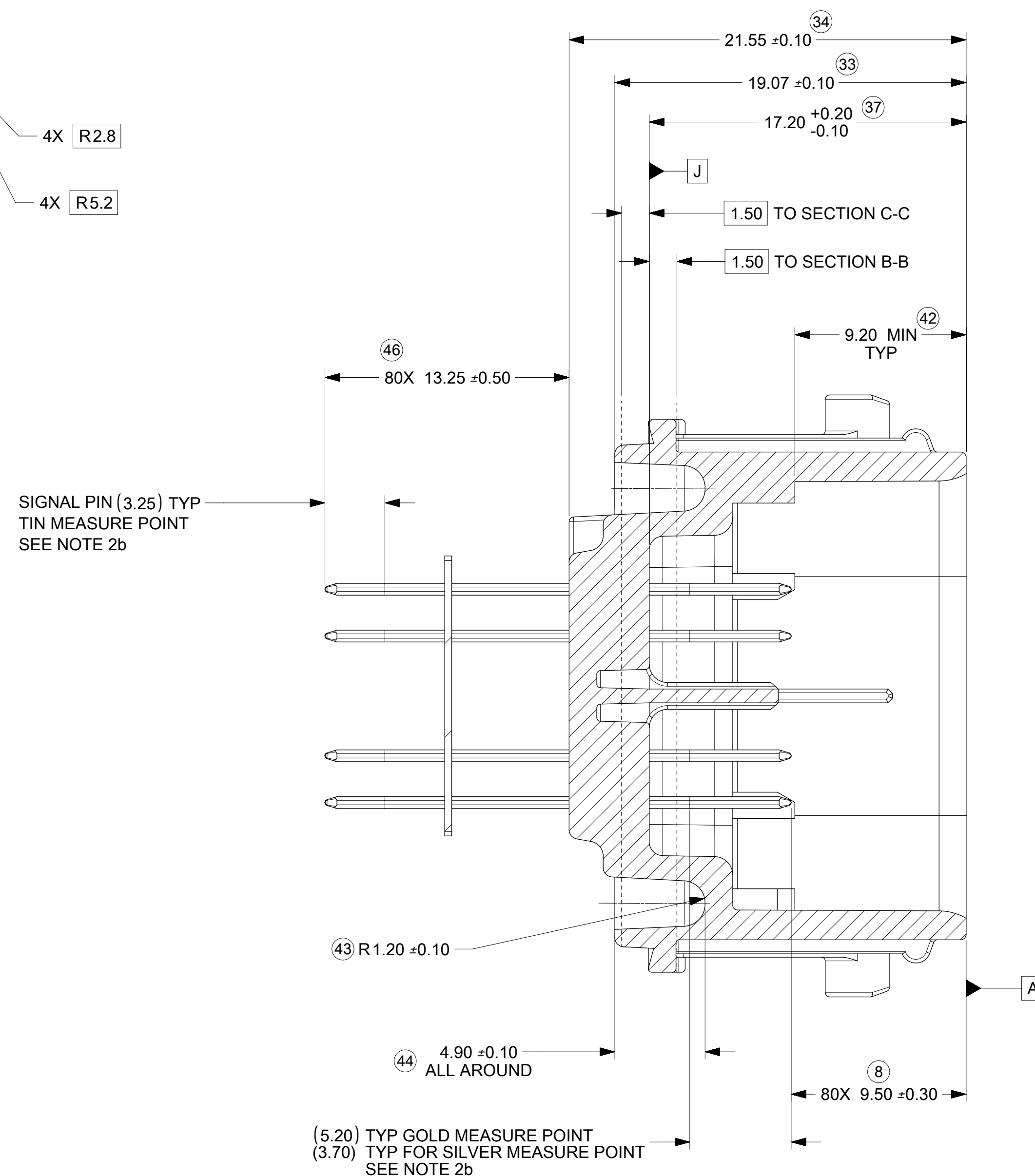
SECTION A-A SCALE 5:1
