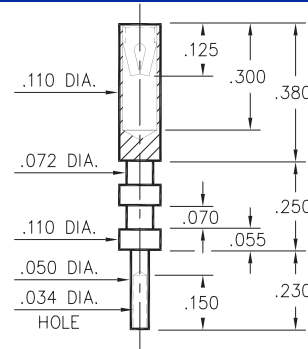
8067-0-19-XX-13-XX-10-0 Wire Termination
