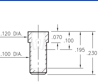
9801-0-15-XX-23-XX-10-0 Solder mount in .102 min. mounting hole
