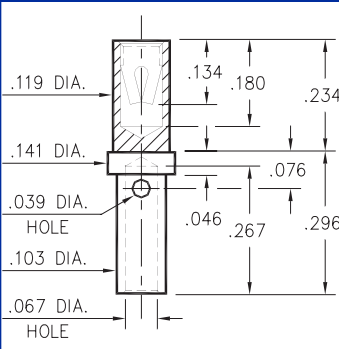
0368-0-33-XX-13-XX-10-0 #16A Crimp Barrel
