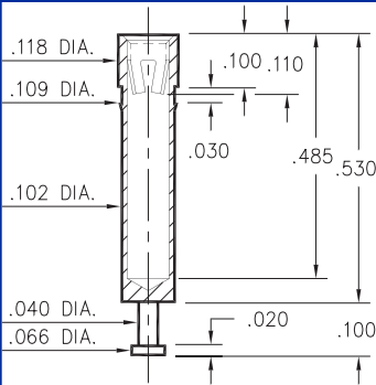
0496-0-15-XX-23-XX-10-0 Press-fit in .106 mounting hole
