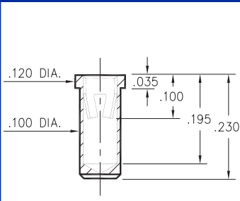
9401-0-15-XX-23-XX-10-0 Solder mount in .102 min. mounting hole
