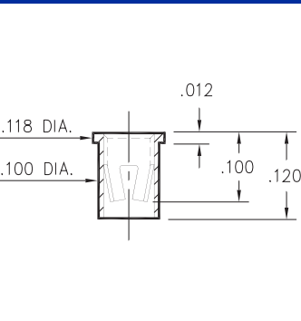
9372-0-15-XX-23-XX-10-0 Solder mount in .102 min. mounting hole
