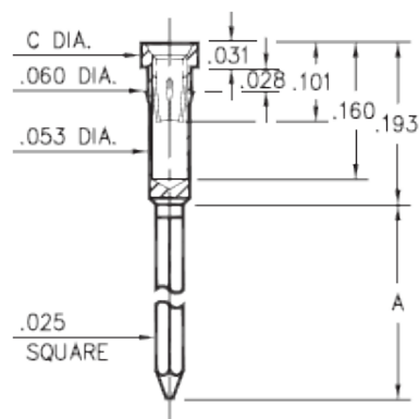
103X-X-17-XX-3X-XX-02-0 Press-fit in .057 mounting hole
